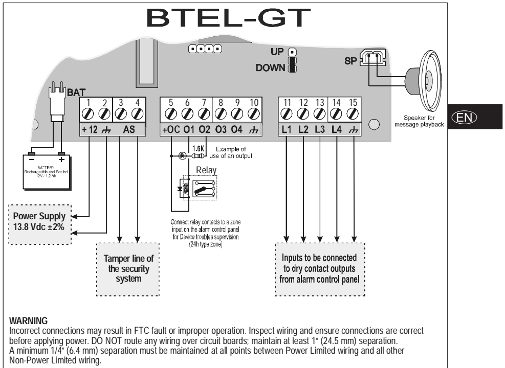
Fig. 3 - Example of connection to the BTEL-GT dialler
